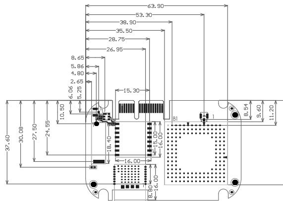
Agora RF Feature Dimensions
