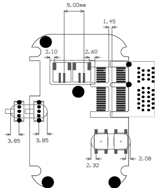
Suggested Layout for Agora (Tectonic Edge™ insertion travel specs)
