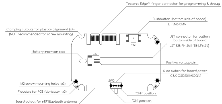
Agora Basic Feature References
