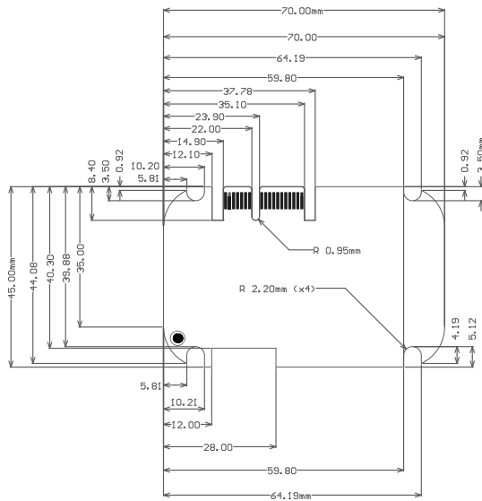
Agora outline dimensions
