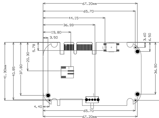
Agora Basic Feature Dimensions
