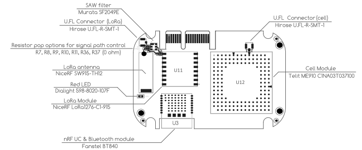
Agora RF Feature Reference
