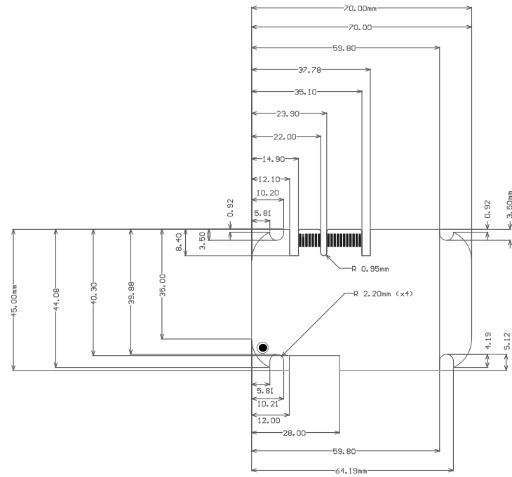
Agora outline dimensions
