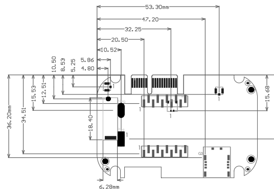
Agora Additional Feature Dimensions
