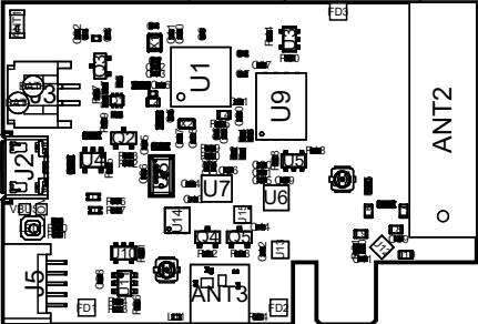
View from Top side (Scale 1:1)
