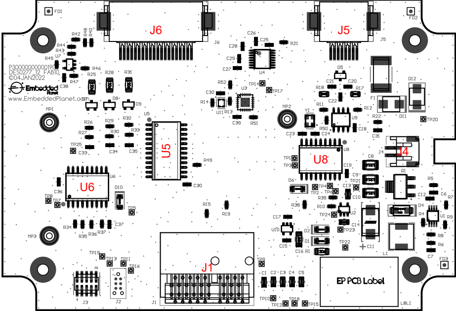
View from Top side (Scale 1:1)
