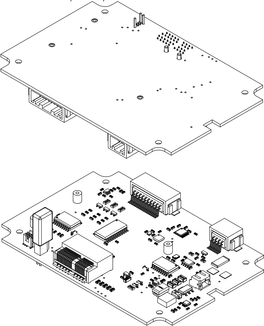
View from Front side (Scale 1:1)
