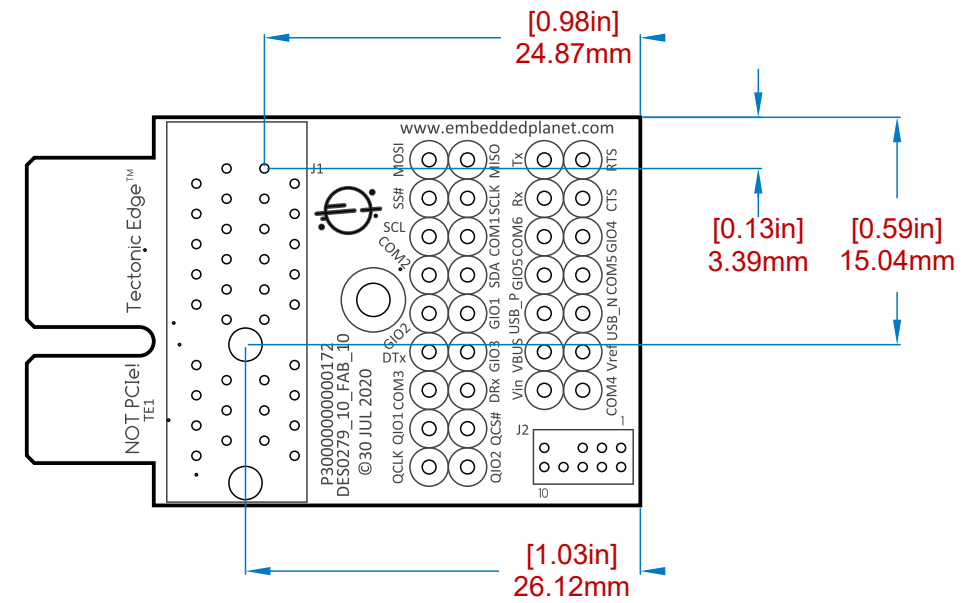
View from Top side (Scale 2:1) (J1 footprint exposed)
